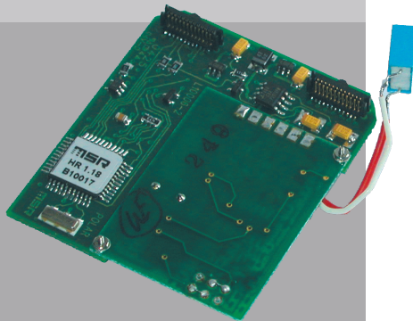
MSR 12 plug-in heart rate module HR
